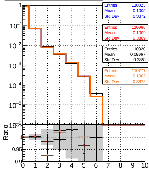
mean hit DOM_mkFit_TTbase DOM_mkFit_TT_retrainOldFiles125_v2_prelimWP_5iter DOM_mkFit_TT_baseline_6iter DOM_mkFit_TT_RetrainV2_WP1_6iter
