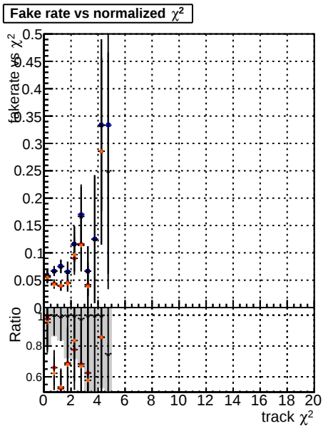
Fake rate vs. Legend: DQM, mkFit, TBase, RetrainOldFiles125_v2_prelimWP_5iter
