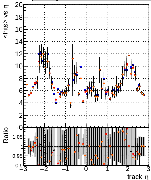
mean hit Legend: - DQM_mkFit_TTbase (blue line) - DQM_mkFit_TT_retrainOldFiles125_v2_prelimWP_5iter (red line with error bars) - DQM_mkFit_TT_baseline_6iter (black line with error bars) - DQM_mkFit_TT_RetrainV2_WP1_6iter (orange line with error bars)
