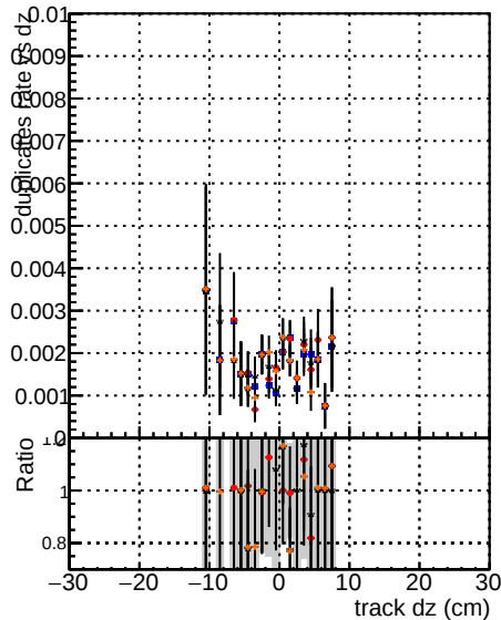
DOM mkFit Ttbase RetrainOldFiles125_v2_prelimWP_5iter RetrainV2_WP1_6iter
