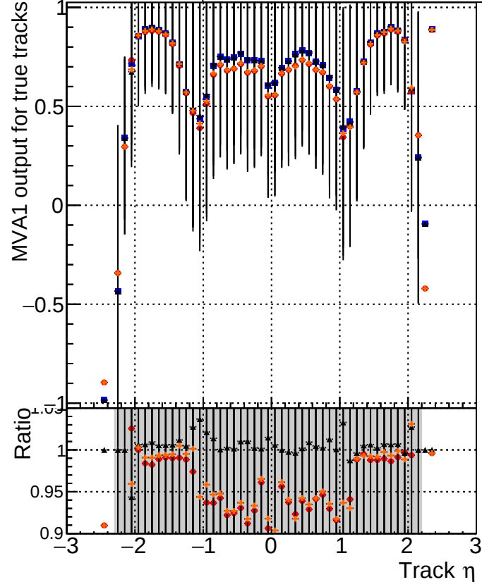
MVA1 of associated tracks (recoToSim) vs. track \eta Legend: DQM_mkFit_TTbase (blue squares) DQM_mkFit_TT_retrainOldFiles125_v2_prelimWP_5iter (red circles) DQM_mkFit_TT_baseline_6iter (black triangles) DQM_mkFit_TT_RetrainV2_WP1_6iter (orange crosses)
