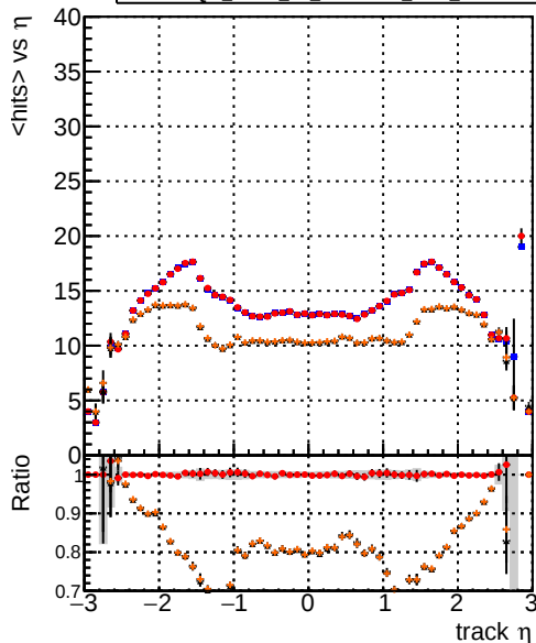
Legend: DQM_mkFit_TTbase (blue), DQM_mkFit_TT_retrainOldFiles125_v2_prelimWP_5iter (red), DQM_mkFit_TT_baseline_6iter (black), DQM_mkFit_TT_RetrainV2_WP1_6iter (orange) mean hit
