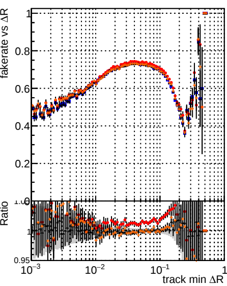
Fake rate vs \Delta R(\text{track, jet}) Legend: DOM mkFit Tbase DOM mkFit RetrainOldFiles125_v2_prelimWP_5iter DOM mkFit RetrainOldFiles125_v2_prelimWP_6iter DOM mkFit RetrainV2_WP1_6iter
