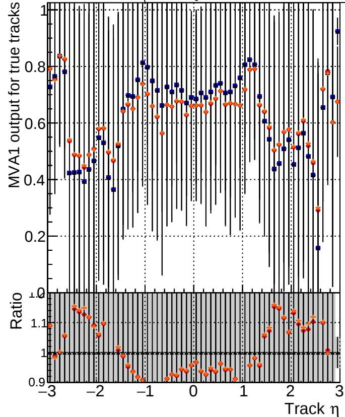
MVA1 of associated tracks (recoToSim) vs. track \eta Legend: ■ DQM_mkFit_TTbase ● DQM_mkFit_TT_retrainOldFiles125_v2_prelimWP_5iter ▲ DQM_mkFit_TT_baseline_6iter ◆ DQM_mkFit_TT_RetrainV2_WP1_6iter
