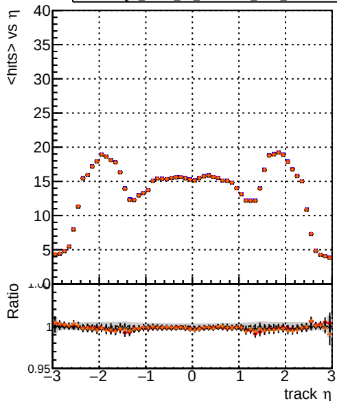
mean hits vs \eta Legend: - DQM_mkFit_TTbase (blue line) - DQM_mkFit_TT_retrainOldFiles125_v2_prelimWP_5iter (red line with dots) - DQM_mkFit_TT_baseline_6iter (black line with dots) - DQM_mkFit_TT_RetrainV2_WP1_6iter (orange line with dots)
