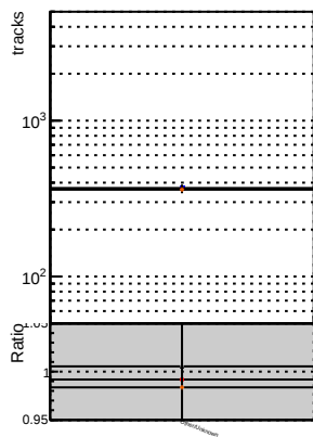
N of reco track vs. \chi^2 for different files
