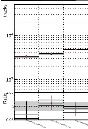
N of reco track vs. \chi^2 for BSM mktFit + Tbase, BSM mktFit + RetrainOldFiles125_v2_prelimWP_5iter, and BSM mktFit + RetrainV2_WP1_6iter
