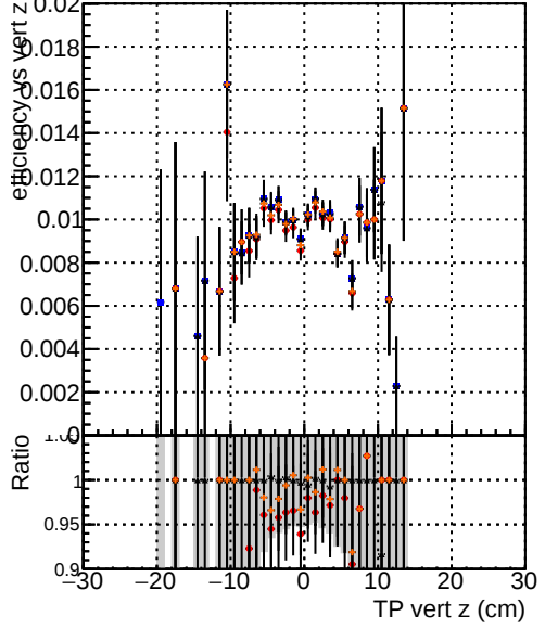
Efficiency vs. TP vert z DOM_mkFit_TTbase DOM_mkFit_TT_retrainOldFiles125_v2_prelimWP_5iter DOM_mkFit_TT_baseline_6iter DOM_mkFit_TT_RetrainV2_WP1_6iter
