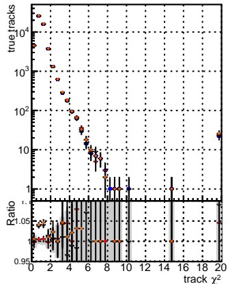
N of reco track vs. \chi^2 for BSM, mFEL, base, and Retrain v2 WP1 5iter
