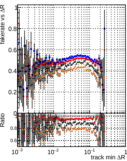
Fake rate vs \Delta R(\text{track, jet}) Legend: DOM mkFit TTbase DOM mkFit retrainOldFiles125_v2_prelimWP_5iter DOM mkFit RetrainOldFiles125_v2_prelimWP_5iter DOM mkFit RetrainV2_WP1_6iter
