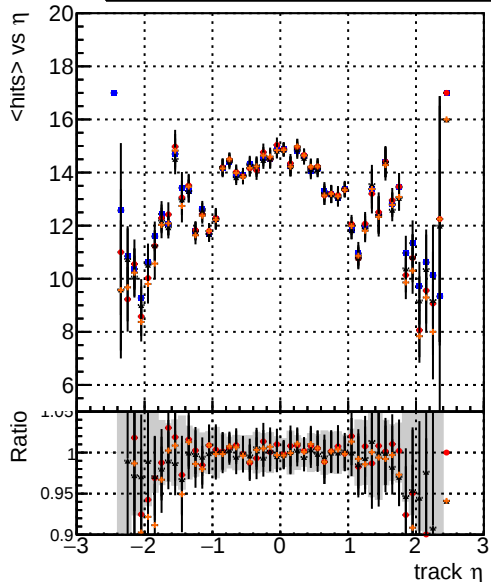
mean hits Legend: - DQM_mkFit_TTbase (blue line) - DQM_mkFit_TT_retrainOldFiles125_v2_prelimWP_5iter (red line with dots) - DQM_mkFit_TT_baseline_6iter (black line with dots) - DQM_mkFit_TT_RetrainV2_WP1_6iter (orange line with dots)
