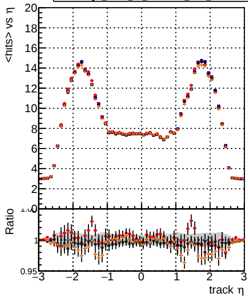
mean hits vs \eta DOM_mkFit_TTbase DOM_mkFit_TT_retrainOldFiles125_v2_prelimWP_5iter DOM_mkFit_TT_baseline_6iter DOM_mkFit_TT_RetrainV2_WP1_6iter
