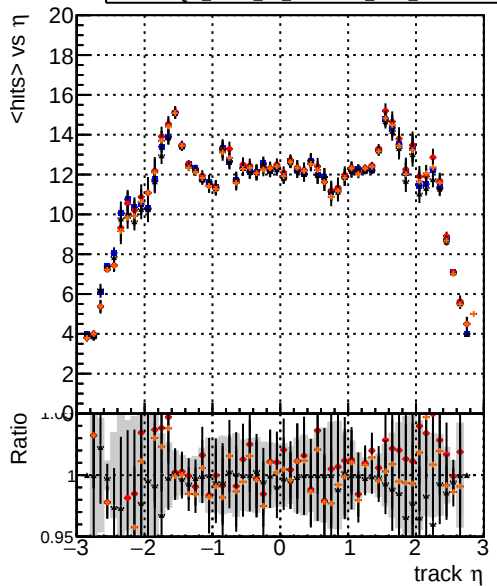
mean hit DOM_mkFit_TTbase DOM_mkFit_TT_retrainOldFiles125_v2_prelimWP_5iter DOM_mkFit_TT_baseline_6iter DOM_mkFit_TT_RetrainV2_WP1_6iter
