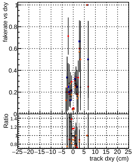
Data (black) Data (red) Data (blue) Data (black) Data (red) Data (blue) Data (black) Data (red) Data (blue)
