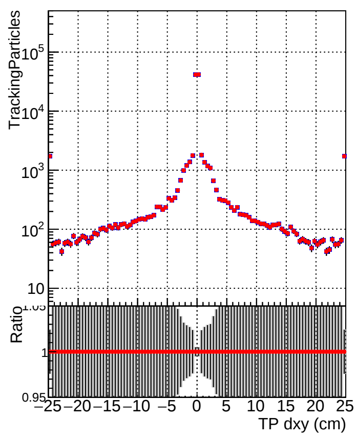
N of simulated track Legend: DQM_mkFit_baseline_lowPT (blue square) DQM_mkFit_baseline6iter_lowPT (red circle)
