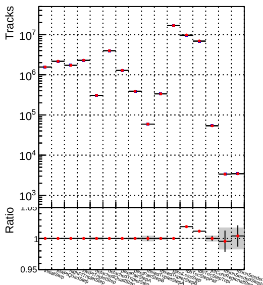
Legend for Number of tracks vs collection: DQM_mkFit_baseline_lowPT DQM_mkFit_baseline6iter_lowPT
