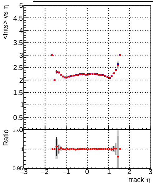
mean hits — DQM_mkFit_baseline_lowPT — DQM_mkFit_baseline6iter_lowPT
