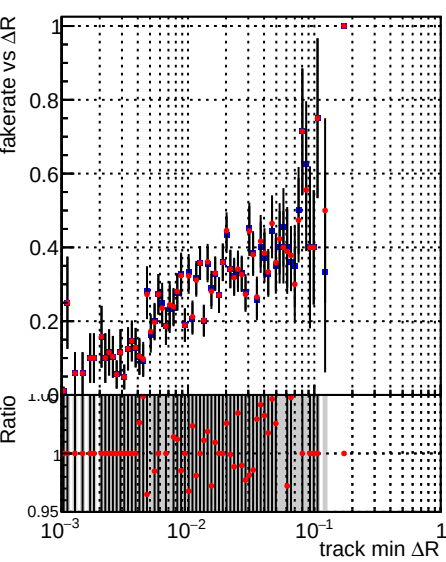
Fake rate vs \Delta R(\text{track, jet}) Legend: —■— DQM_mkFit_baseline_lowPT —●— DQM_mkFit_baseline6iter_lowPT
