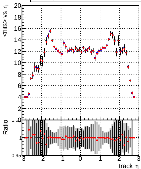
mean hits — DQM_mkFit_baseline_lowPT — DQM_mkFit_baseline6iter_lowPT
