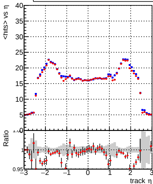
mean hit — DQM_mkFit_baseline_lowPT — DQM_mkFit_baseline6iter_lowPT
