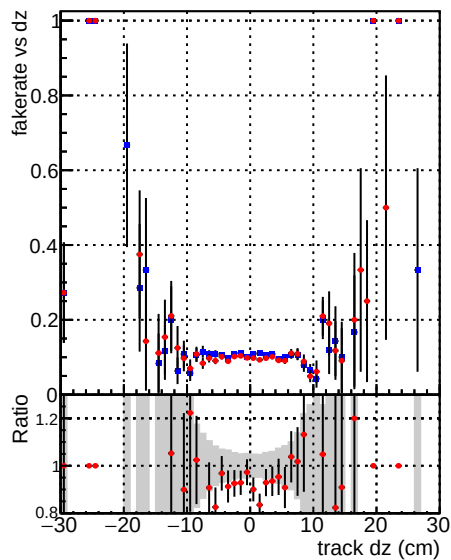
Fake rate vs dz Legend: DQM mkFit baseline_lowPT (blue squares) DQM mkFit baseline6iter_lowPT (red circles)
