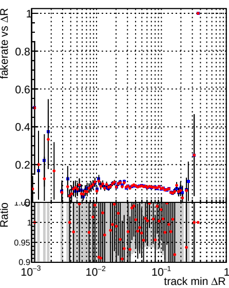
Legend: \blacksquare DQM_mkFit_baseline_lowPT \bullet DQM_mkFit_baseline6iter_lowPT
