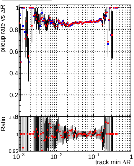
Legend: \blacksquare DQM_mkFit_baseline_lowPT \bullet DQM_mkFit_baseline6iter_lowPT
