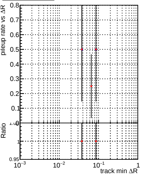
Legend: DQM_mkFit_baseline_lowPT (blue dots), DQM_mkFit_baseline6iter_lowPT (red dots)
