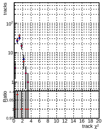
N of reco track vs. \chi^2 for DQM mkFit baseline_lowPT and DQM mkFit baseline6iter_lowPT
