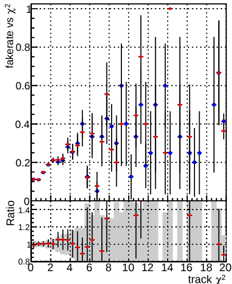
Fake rate vs. —●— DQM_mkFit_baseline_lowPT —●— DQM_mkFit_baseline6iter_lowPT
