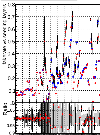
Fake rate vs. —●— DQM mkFit baseline_lowPT —●— DQM mkFit baseline6iter_lowPT
