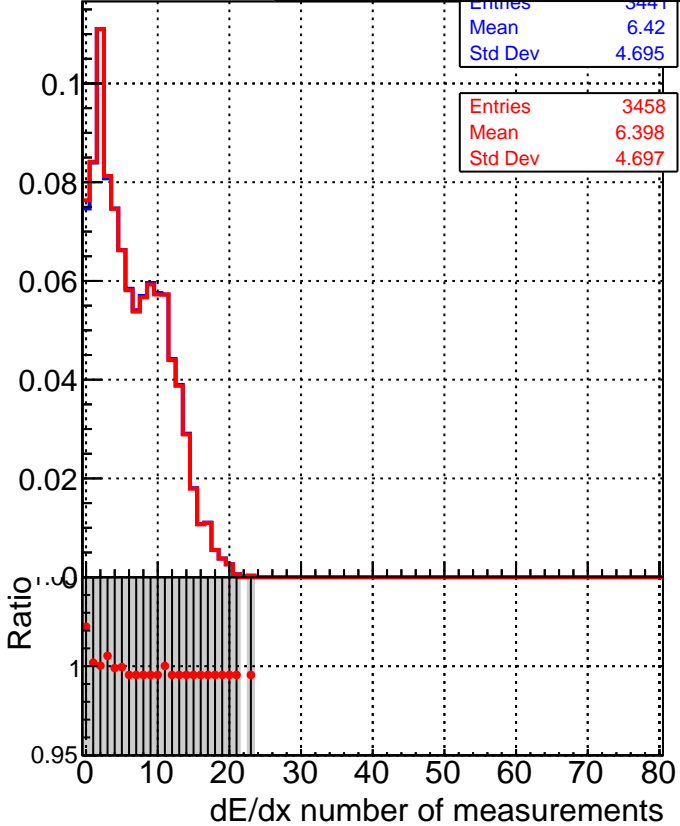
—■ DQM_mkFit_baseline_lowPT —● DQM_mkFit_baseline6iter_lowPT
