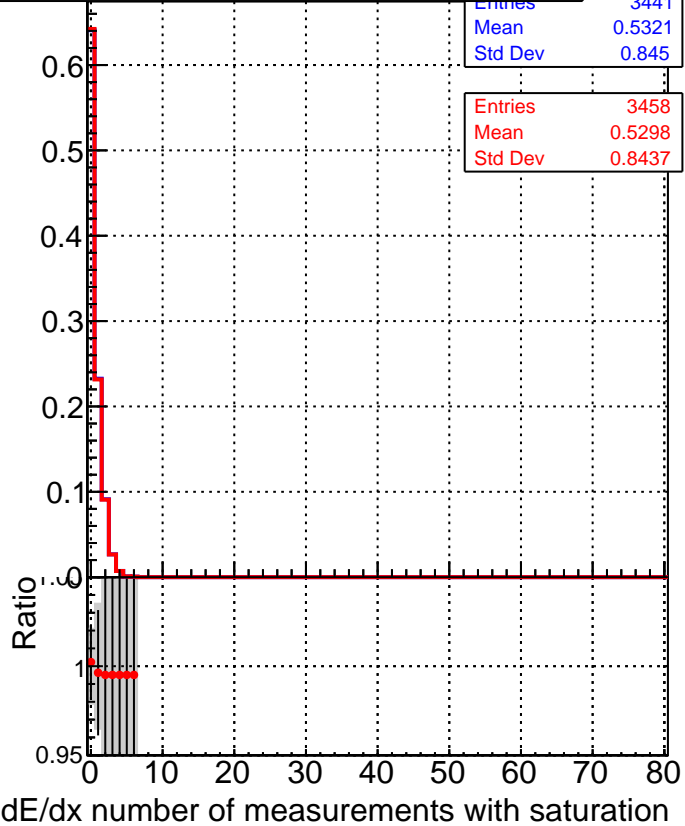
—■ DQM_mkFit_baseline_lowPT —● DQM_mkFit_baseline6iter_lowPT
