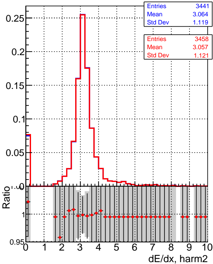
—■ DQM_mkFit_baseline_lowPT —● DQM_mkFit_baseline6iter_lowPT
