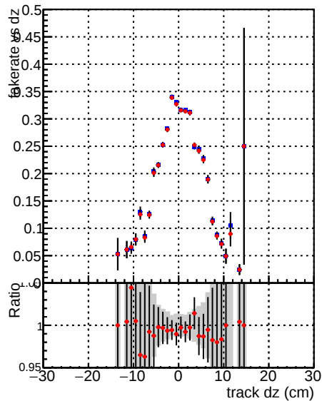
Fake rate vs dz —●— DQM_mkFit_baseline_lowPT —●— DQM_mkFit_baseline6iter_lowPT
