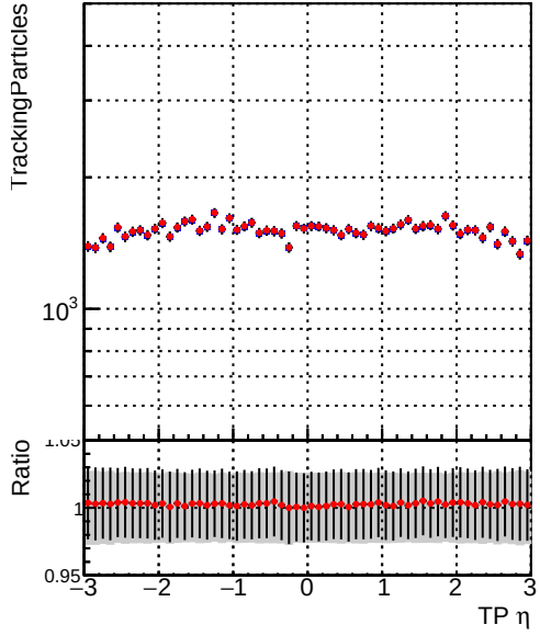
Legend: DQM_mkFit_baseline_lowPT (blue line with dots), DQM_mkFit_baseline6iter_lowPT (red line with dots)
