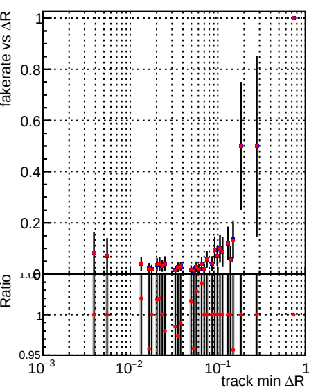
Legend: DQM_mkFit_baseline_lowPT (grey squares), DQM_mkFit_baseline6iter_lowPT (red circles)
