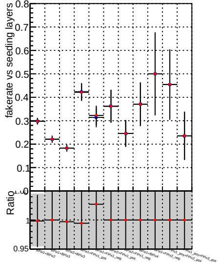
Fake rate vs. Legend: DQM_mkFit_baseline_lowPT DQM_mkFit_baseline6iter_lowPT
