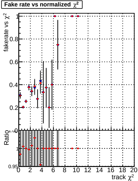
Fake rate vs. Legend: DQM_mkFit_baseline_lowPT DQM_mkFit_baseline6iter_lowPT
