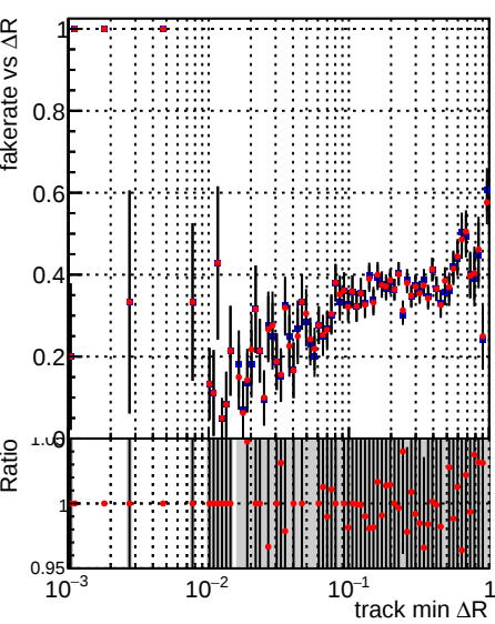
Fake rate vs \Delta R (track, jet) DQM_mkFit_baseline_lowPT (blue squares) DQM_mkFit_baseline6iter_lowPT (red circles)
