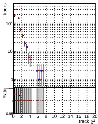
N of reco track vs. \chi^2 —●— DQM_mkFit_baseline_lowPT —●— DQM_mkFit_baseline6iter_lowPT
