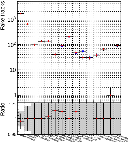
Number —●— DQM_mkFit_baseline6iter_lowPT
