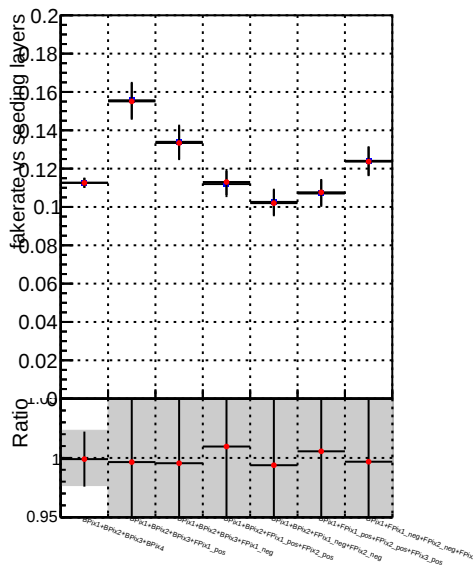
Fake rate vs. DQM_mkFit_baseline_lowPT DQM_mkFit_baseline6iter_lowPT
