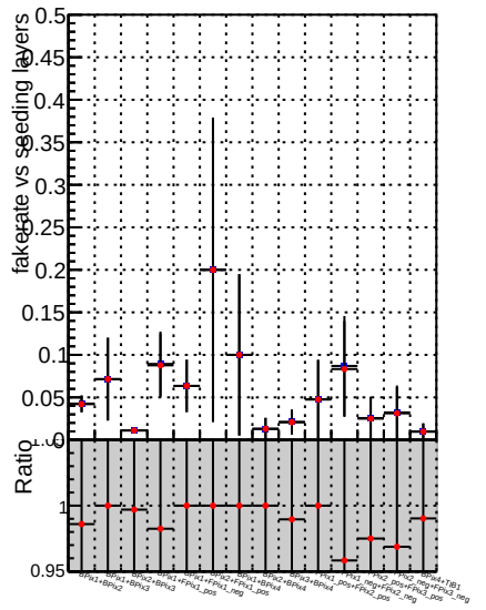
Fake rate vs. —•— DQM_mkFit_baseline_lowPT —•— DQM_mkFit_baseline6iter_lowPT
