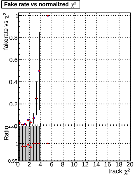
Fake rate vs. —•— DQM_mkFit_baseline_lowPT —•— DQM_mkFit_baseline6iter_lowPT
