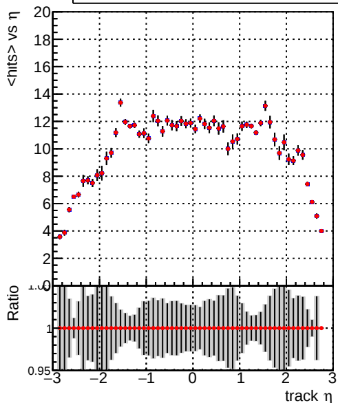
mean hit — DQM_mkFit_baseline_lowPT — DQM_mkFit_baseline6iter_lowPT
