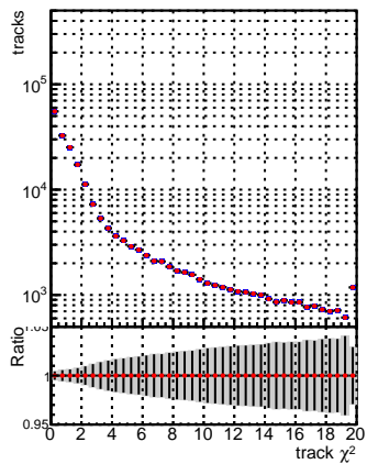
Legend: DQM_mkFit_baseline_lowPT (blue line), DQM_mkFit_baseline6iter_lowPT (red line)
