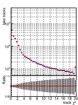
Legend: DQM_mkFit_baseline_lowPT (blue line), DQM_mkFit_baseline6iter_lowPT (red line)
