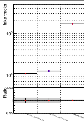
N of fake tracks vs. \chi^2
