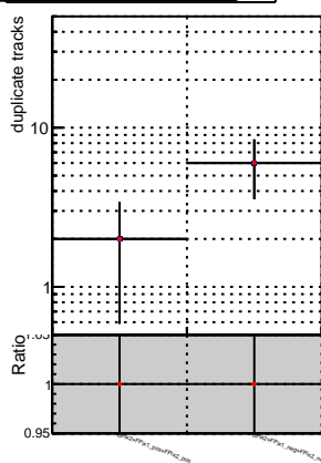
N of duplicate tracks vs. \chi^2
