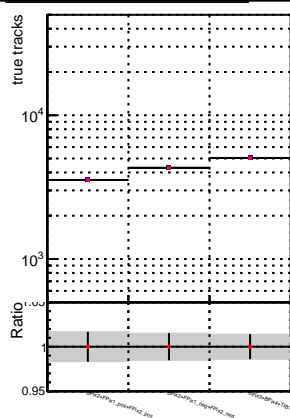
N of associated (recoToSim) tracks vs. \chi^2
