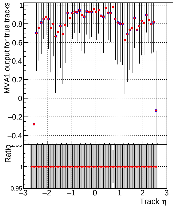
MVA1 of associated tracks (recoToSim) vs. track \eta Legend: ■ DQM_mkFit_baseline_lowPT ● DQM_mkFit_baseline6iter_lowPT
