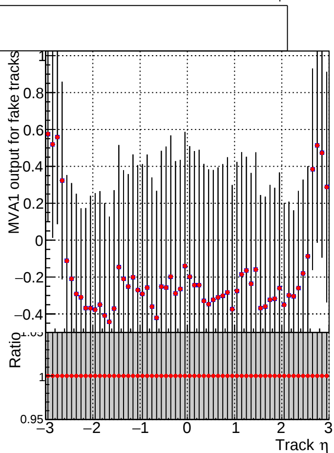
MVA1 of associated tracks (recoToSim) vs. track \eta ■ DQM_mkFit_baseline_lowPT ● DQM_mkFit_baseline6iter_lowPT
