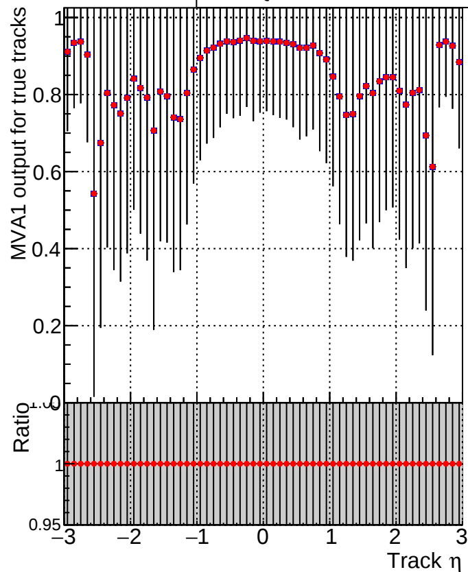
MVA1 of associated tracks (recoToSim) vs. track \eta ■ DQM_mkFit_baseline_lowPT ● DQM_mkFit_baseline6iter_lowPT
