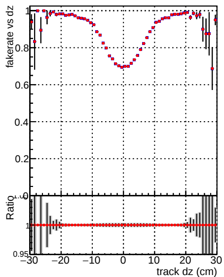
—●— DQM_mkFit_baseline_lowPT —●— DQM_mkFit_baseline6iter_lowPT
