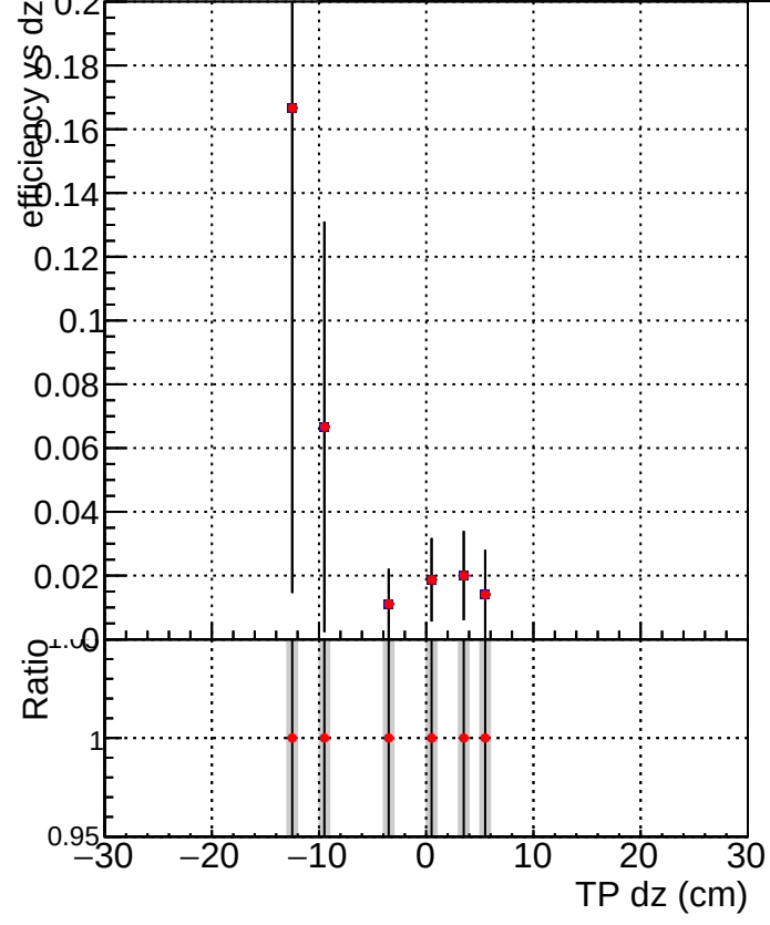
Efficiency vs Dz Legend: DQM_mkFit_baseline_lowPT (Blue square) DQM_mkFit_baseline6iter_lowPT (Red circle)
