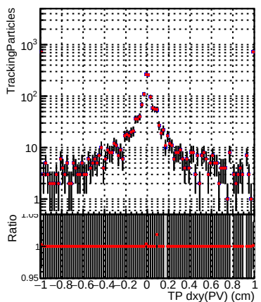
N of sim DQM_mkFit_baseline_lowPT
