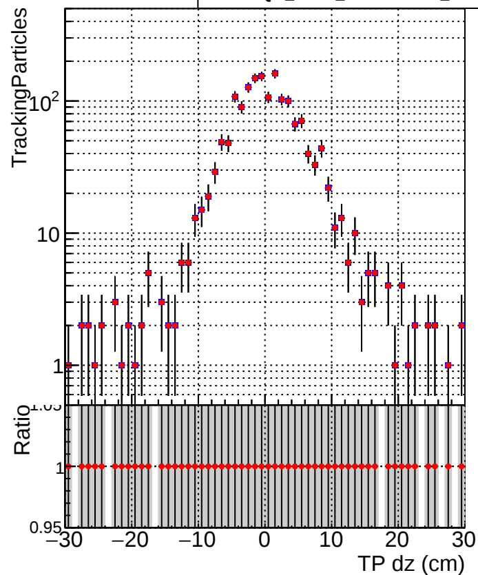
N of simulated track Legend: DQM_mkFit_baseline_lowPT DQM_mkFit_baseline6iter_lowPT
