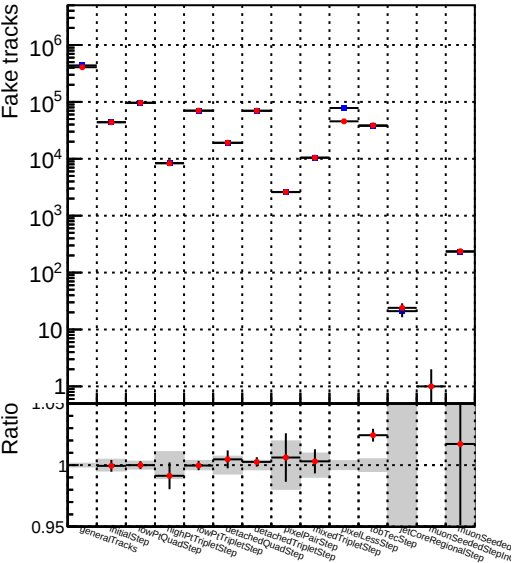
Number —●— DQM_mkFit_baseline6iter_lowPT
