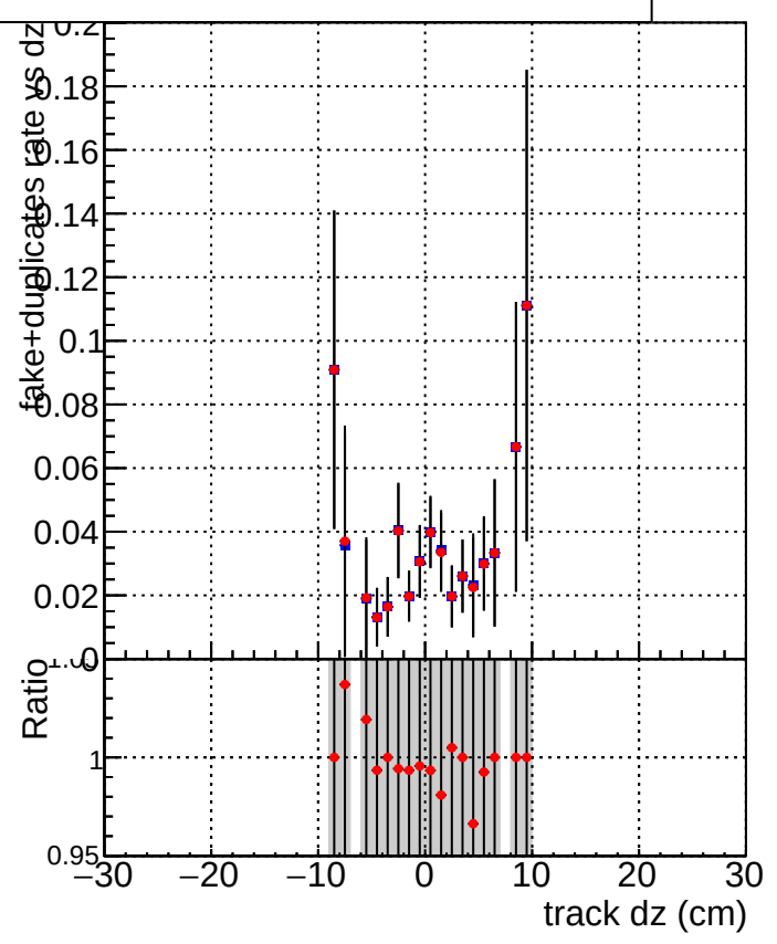
Legend: DQM_mkFit_baseline_lowPT (blue square), DQM_mkFit_baseline6iter_lowPT (red circle)
